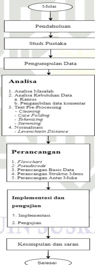
Gambar 3. 1 Metedologi Penelitian
