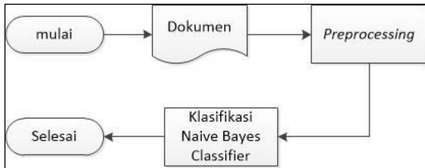
Gambar 3. 2 Analisa flowchart
