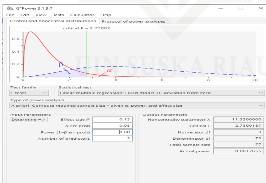
Gambar 3. 1 Hasil Sampel Gpower
