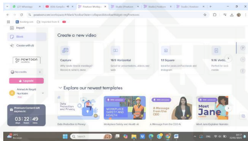
Gambar II. 10 Menu Blank
