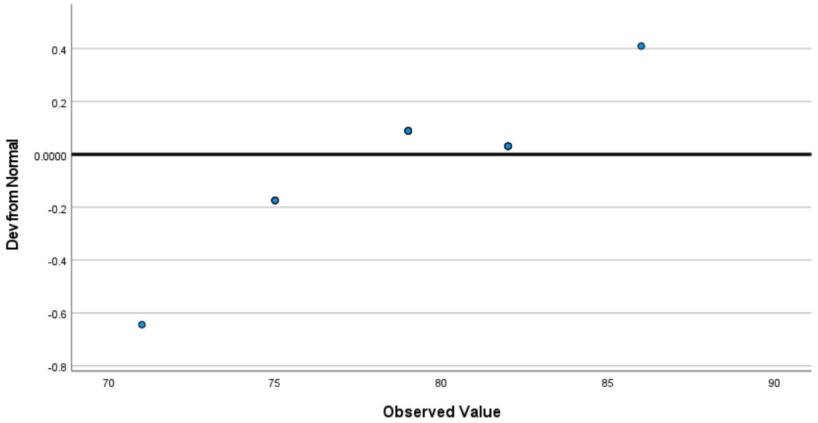
Detrended Normal Q-Q Plot of Hasil Menulis Cerpen Siswa for Kelas= Post-Test Kelas Kontrol
