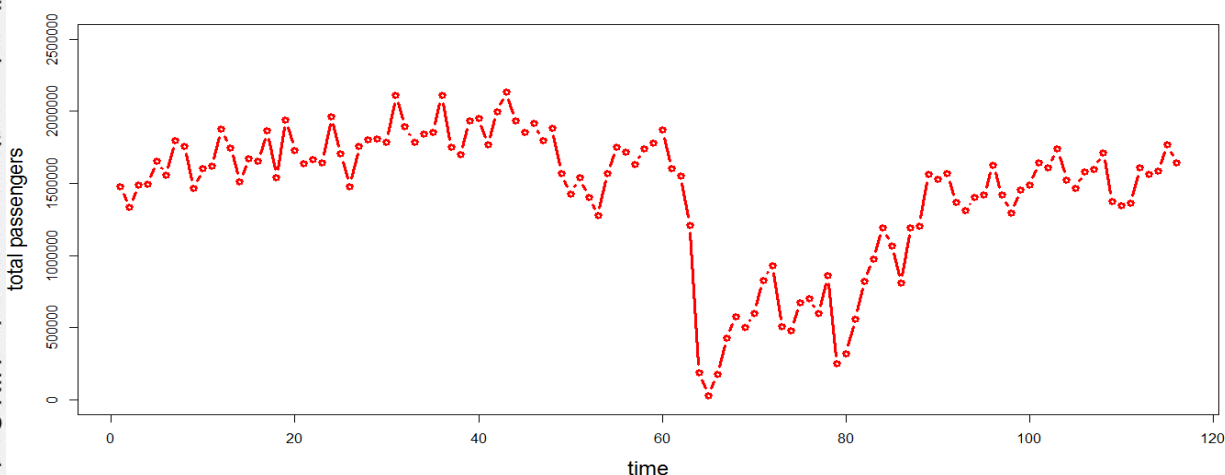
Figure 1. Plot of the Number of Airplane Passengers
