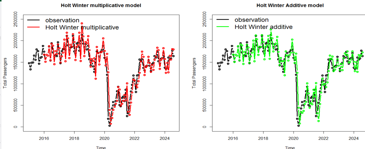
Figure 4. Comparison of Actual Data and Predicted Data from the Holt Winters Additive and Multiplicative Model
