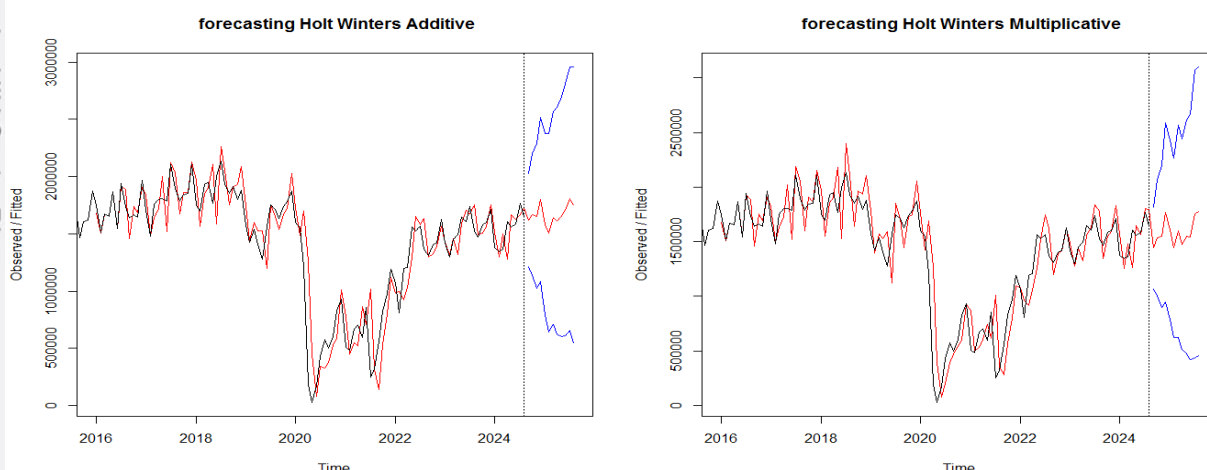
Figure 5. Comparison of The forecasting for a 12 month by Holt Winter Additive and Multiplicative Models
