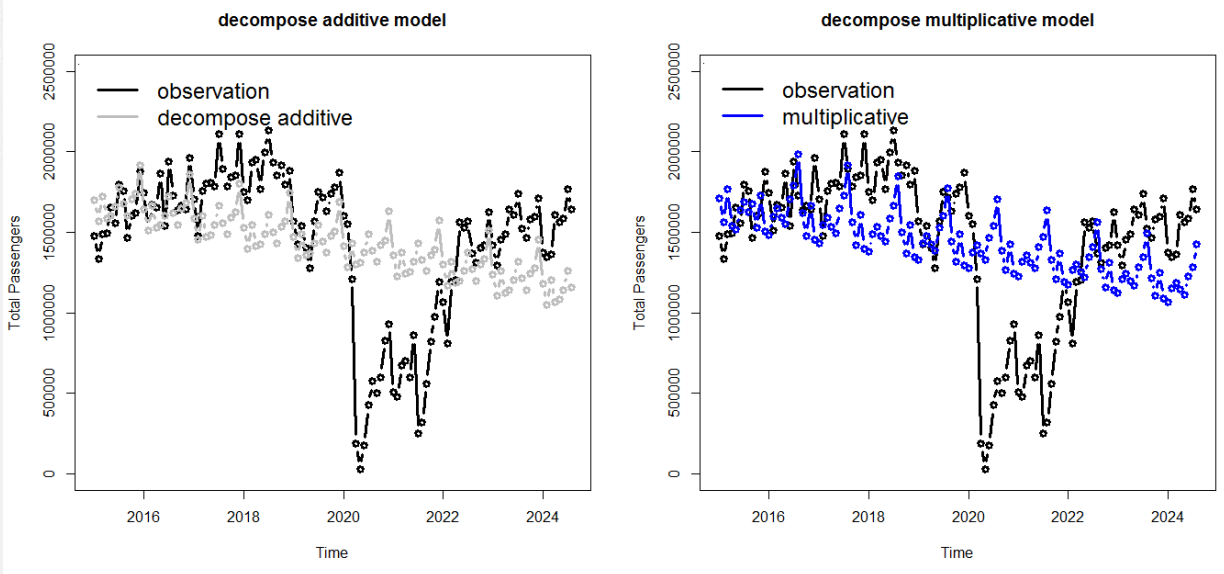
Figure 3. Comparison of Actual Data and Predicted Data from the Decompose Additive and Multiplicative Model
