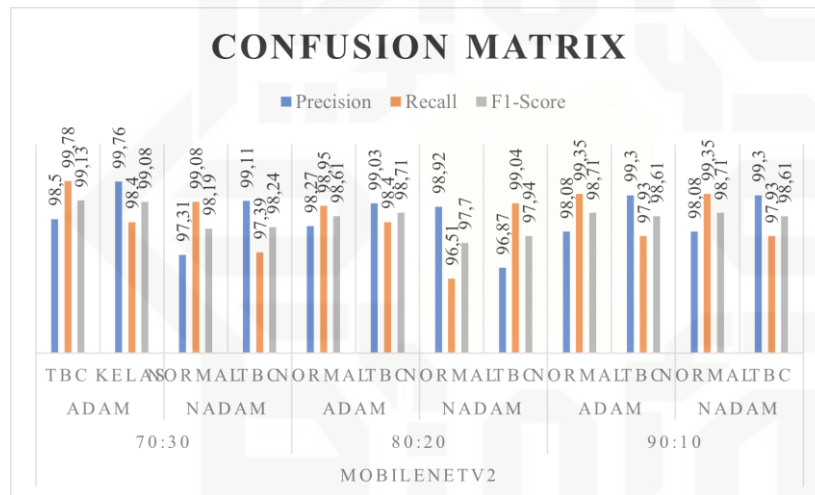
Gambar 11. Hasil Confusion Matrix MobileNetV2
