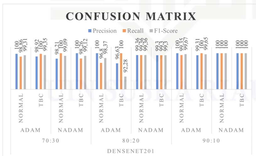
Gambar 9. Hasil Confusion Matrix DenseNet201
