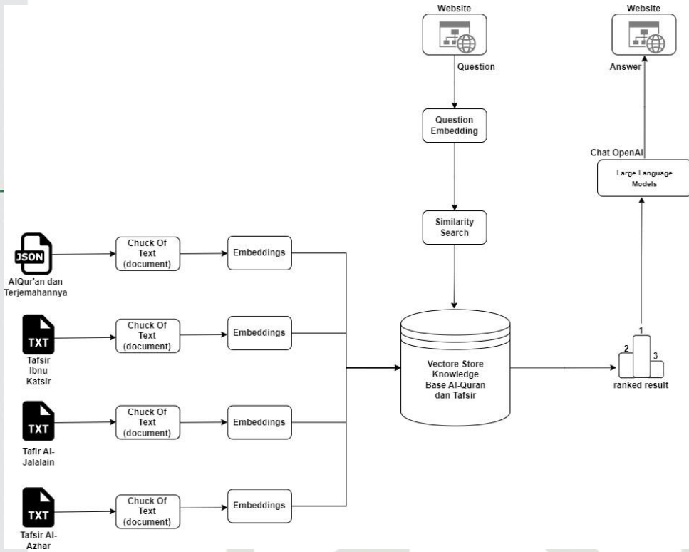
Gambar 2 Diagram Alir Question Answering System
