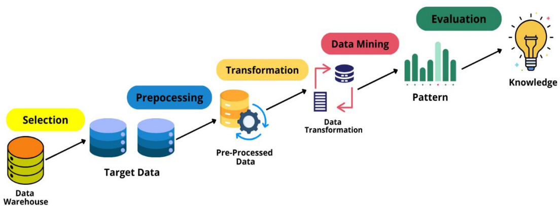
Gambar 2.1 Tahapan Knowledge Discovery in Database (KDD)
