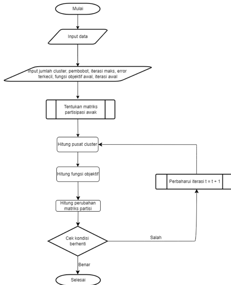
Gambar 3.2 Flowchart Algoritma Fuzzy C-Means
