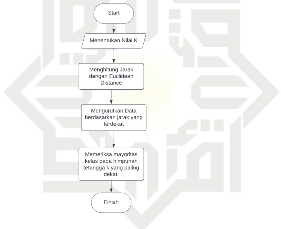
Gambar 3.2 Alur K-Nearest Neighbor (K-NN)
