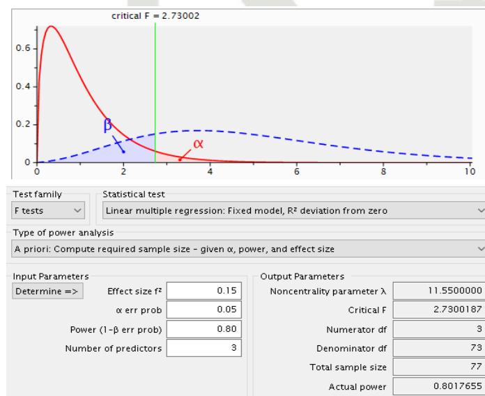
Gambar 3.1 Hasil G*Power
