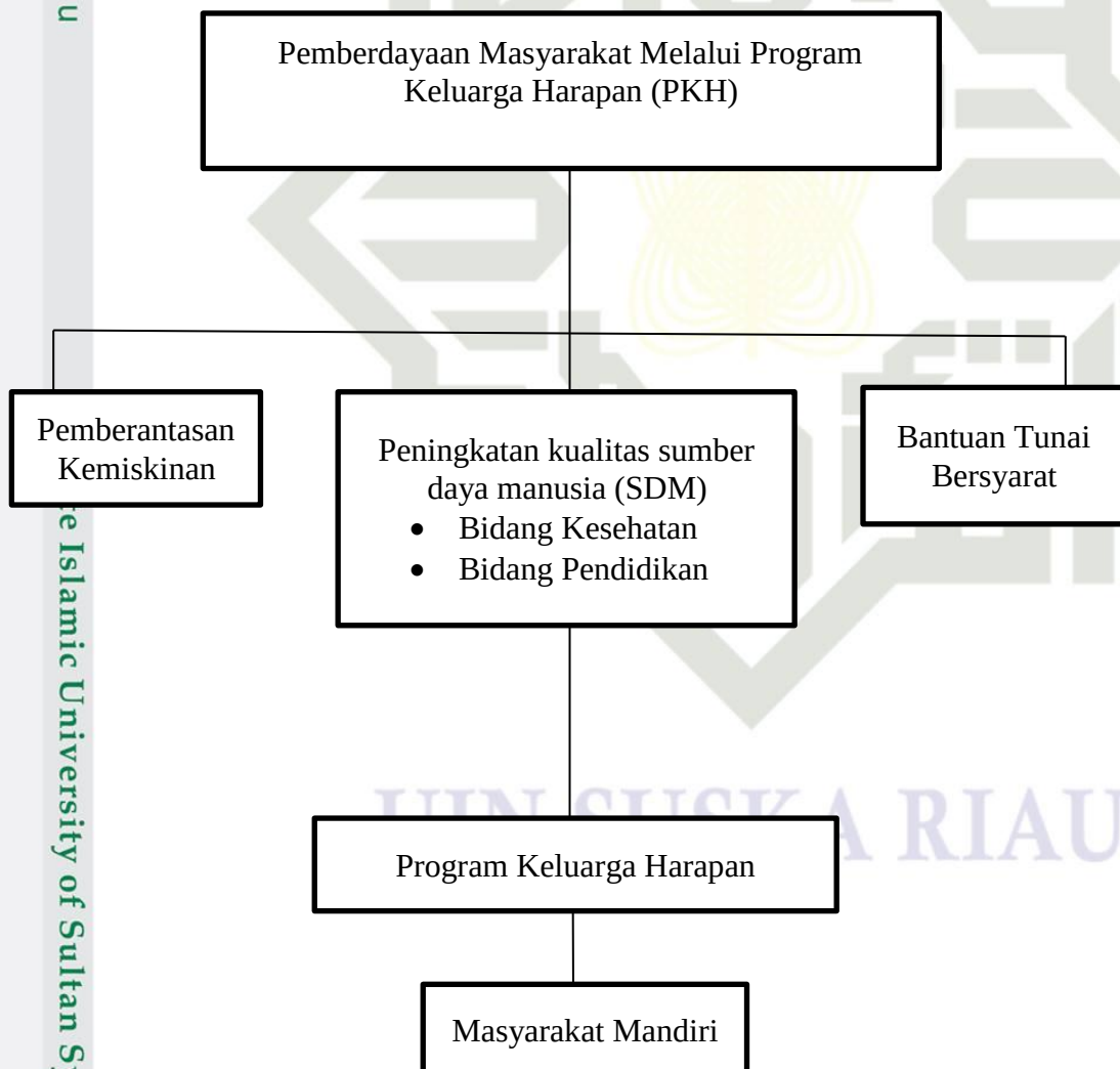
Gambar 2.1 Indikator Penelitian
