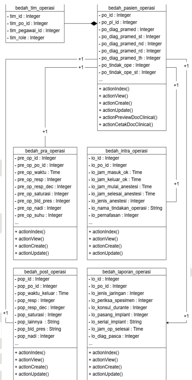
Figure 6. Class Diagram
