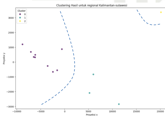
Gambar 4. scatter plot Klasterisasi Regional Kalimantan-Sulawesi.
