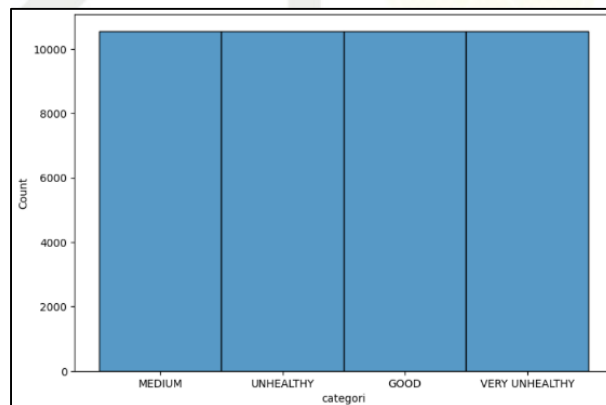
Fig 4: After Oversampling
