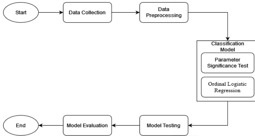
Fig 1: Research Methodology
