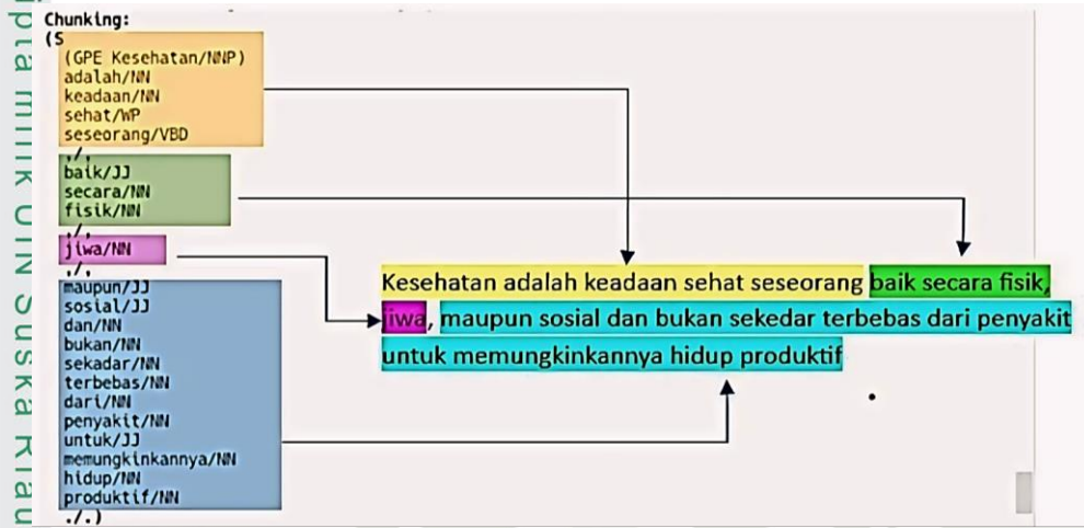
Gambar 3. Hasil Chunking
