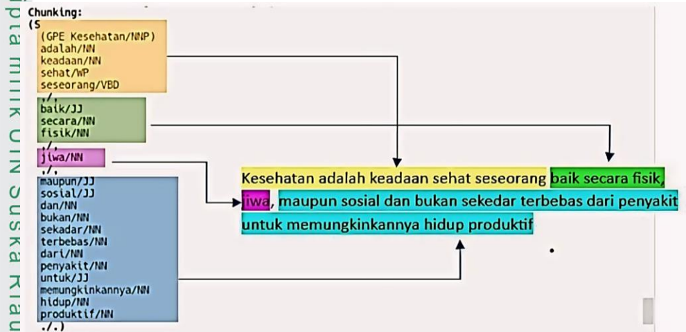
Gambar 3. Hasil Chunking
