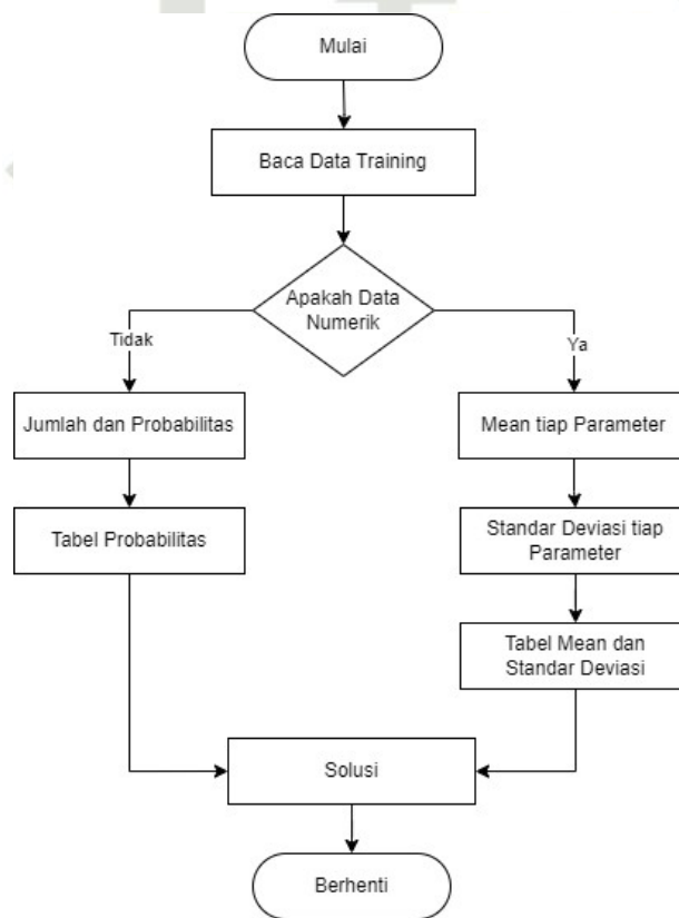
Gambar 3. 2 Alur Metode Naive Bayes
