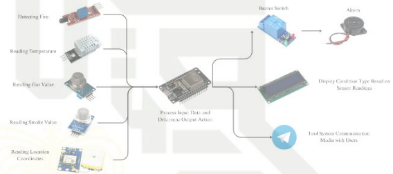
Figure 1. Overview of the Gas Leak and Fire Detection System
