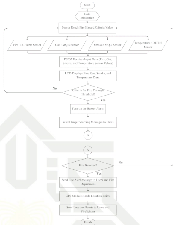
Figure 3. Flowchart Gas Leak and Fire Detection System
