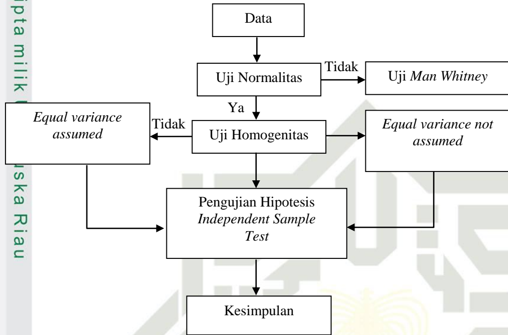
Gambar III.1 Alur pengujian Hipotesis
