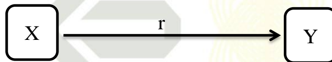
Gambar III.1 Hubungan Antar Variabel
