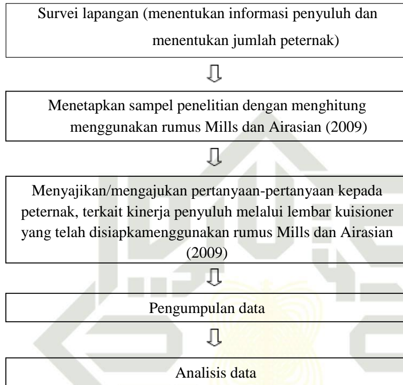
Gambar 3.1 Prosedur penelitian
