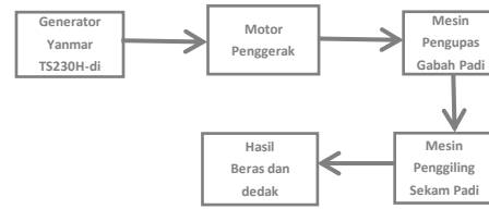
Figure 1. Rice Grain Processing Scheme
