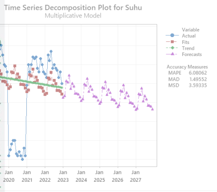
Figure 12 Time Series Decomposition Plot for Temperature
