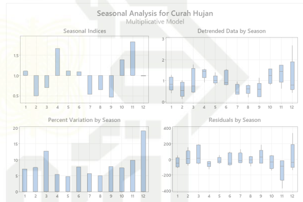
Figure 9 Seasonal Analysis for Rainfall
