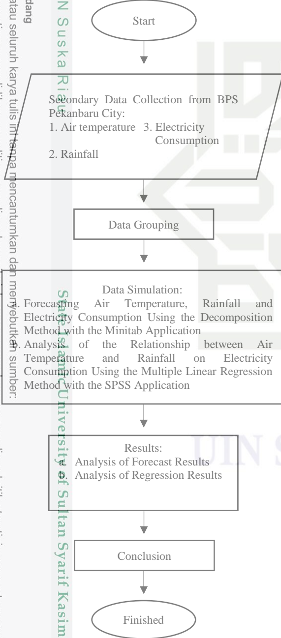
Figure 1 Research Flowchart
