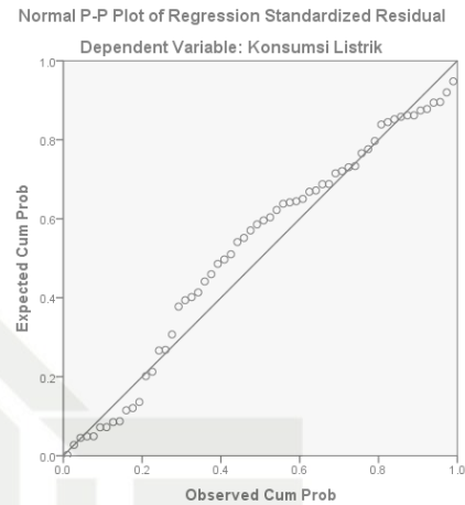
Figure 11 Normal P –P Plot
