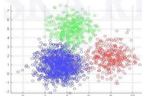
Gambar 3. K-means clustering
