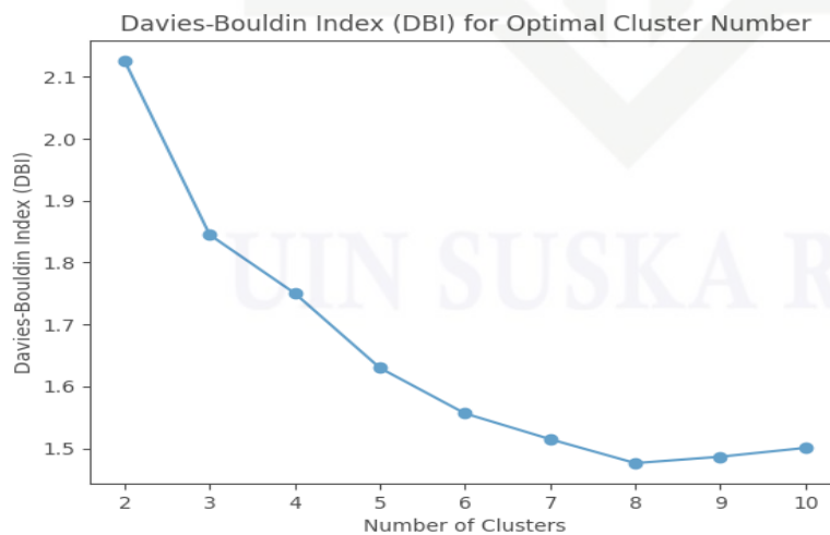
Gambar 4. Davies-Bouldin Index (DBI)
