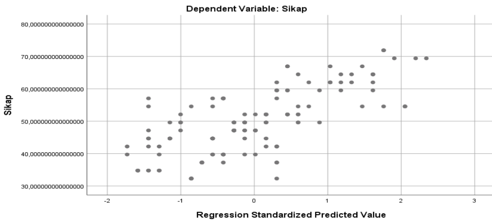
Scatterplot
