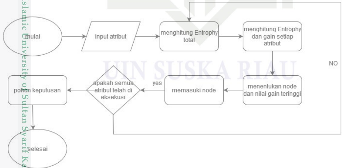
Gambar 2 .Flowchart Algoritma
