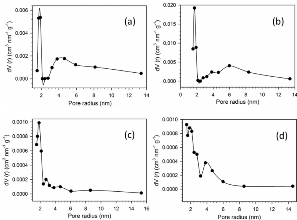
Figure 7. Pore distribution of PCE samples.
