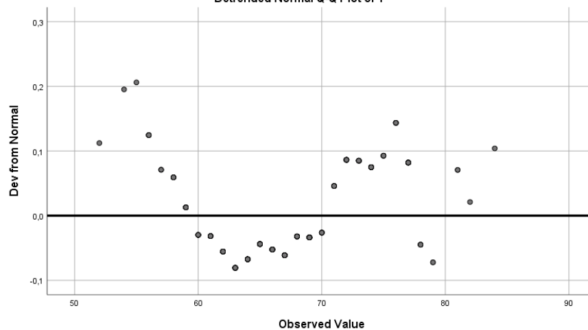
Detrended Normal Q-Q Plot of Y
