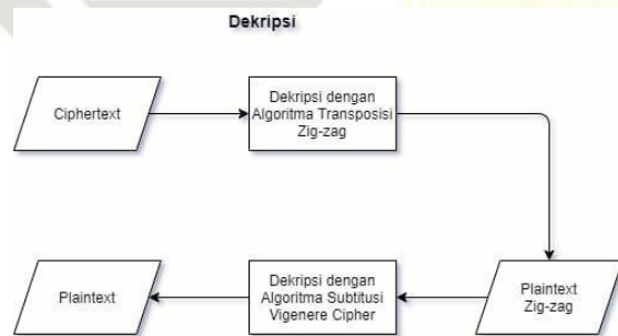
Gambar 4. Flowchart Dekripsi
