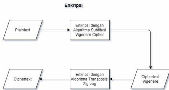
Gambar 3. Flowchart Enkripsi
