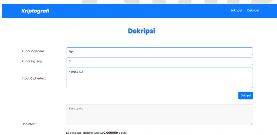
Gambar 7. Proses Dekripsi
