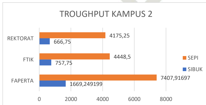
Gambar 5. Grafik Nilai Throughput Kampus 2
