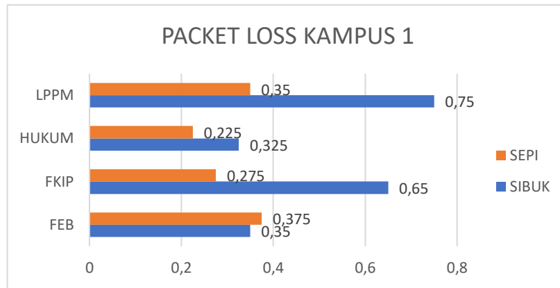
Gambar 6. Grafik Nilai Packet Loss Kampus 1
