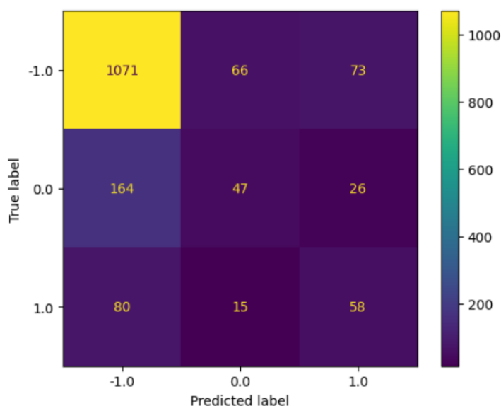
Gambar 8: Confusion Matrix
