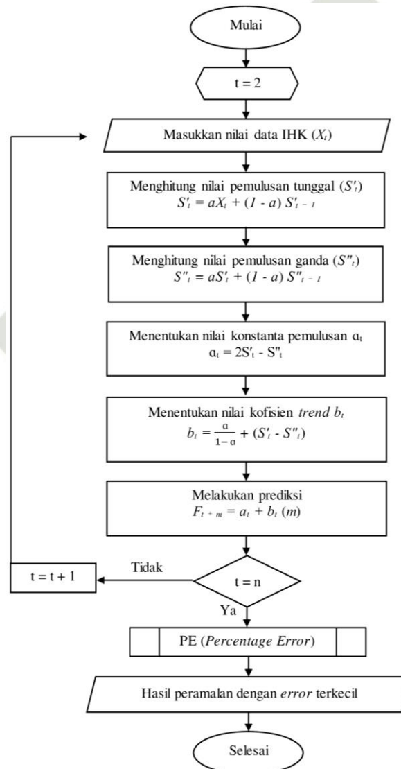
Gambar 1 Tahapan Metode Double Exponential Smoothing
