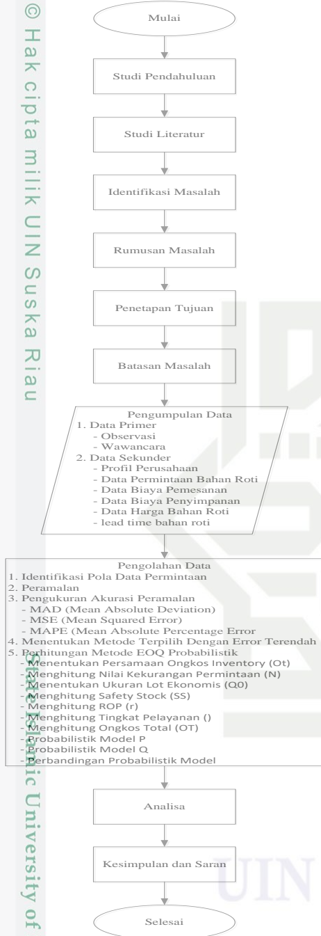
Gambar 1. Flowchart Penelitian
