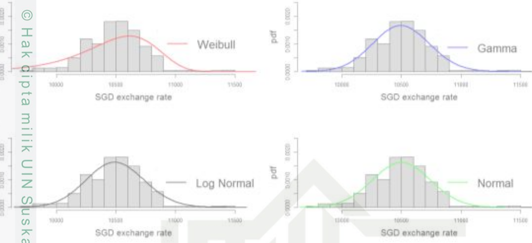
Fig. 3. A plot of the histogram and theoretical Weibull densities (red line), Gamma densities (blue line), Log Normal (black line) and Normal (green line) for the exchange rate between the Singapore Dolar (SGD) and Indonesia Rupiah (IDR)
