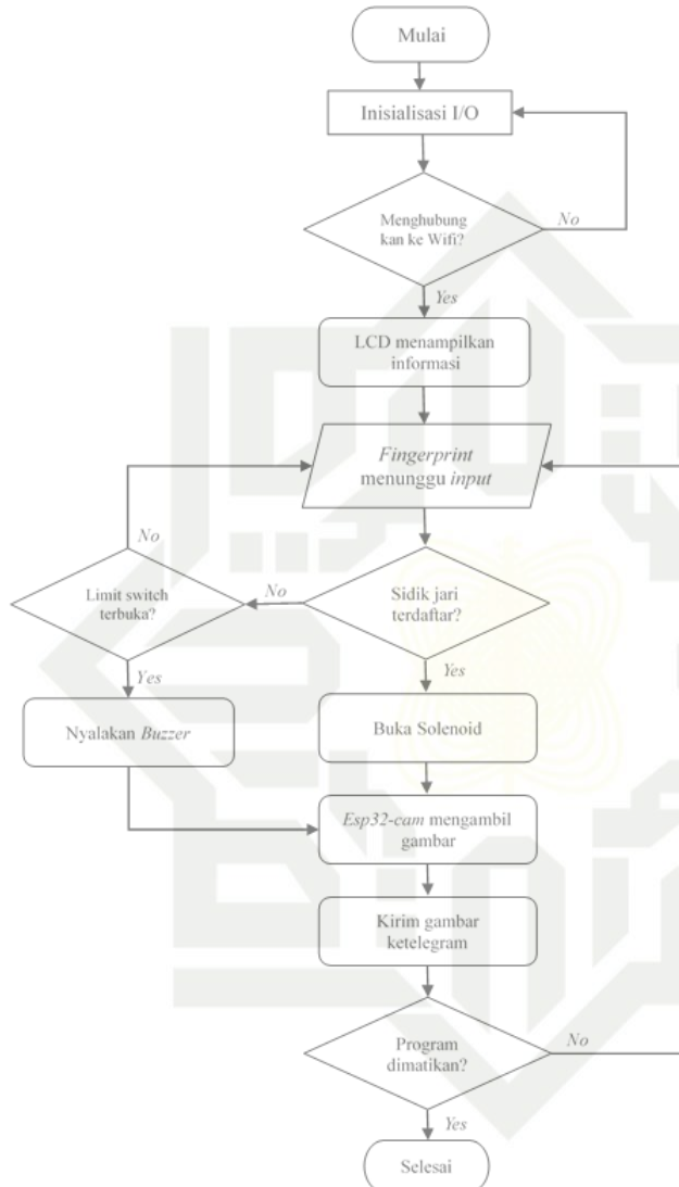
Gambar 4. Flowchart Sistem
