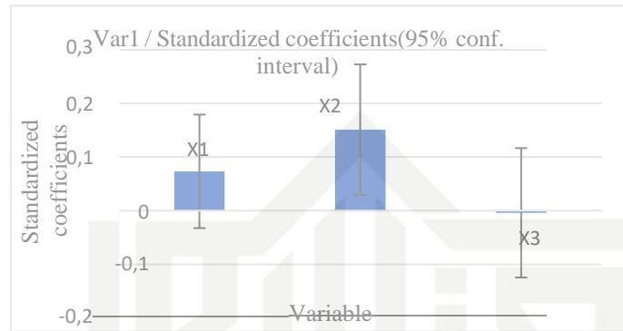
Gambar 2. Standardized Coefficients
