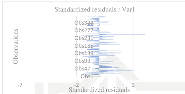
Gambar 6. Standardized Residuals
