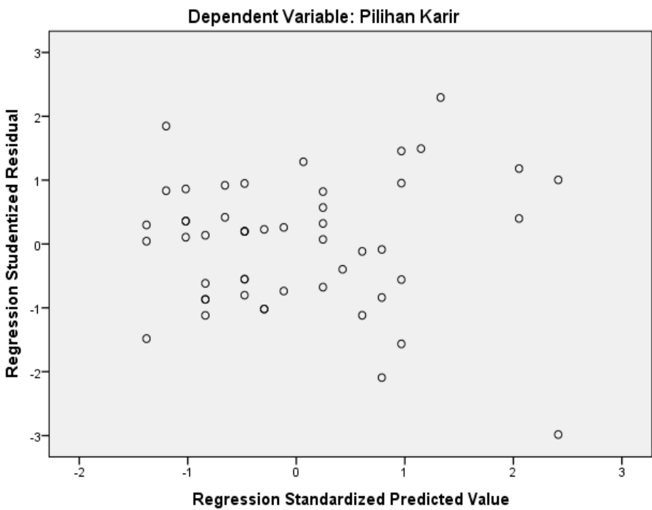
Scatterplot
