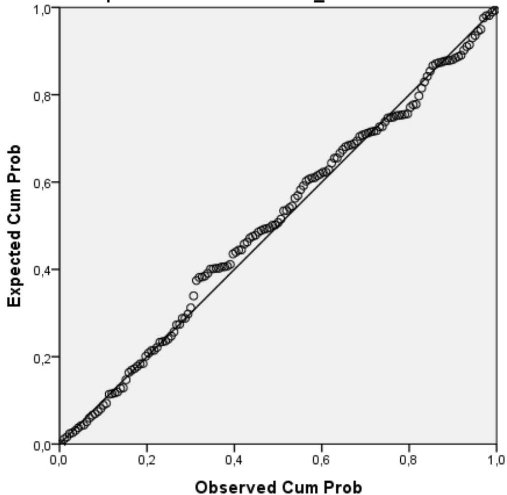
Gambar Scater Plot Normalitas Variabel Dependent dan Independent
