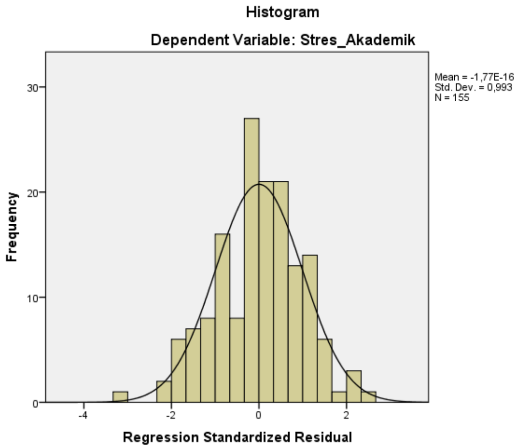
Gambar Histogram Variabel Dependent dan Variabel Independent
