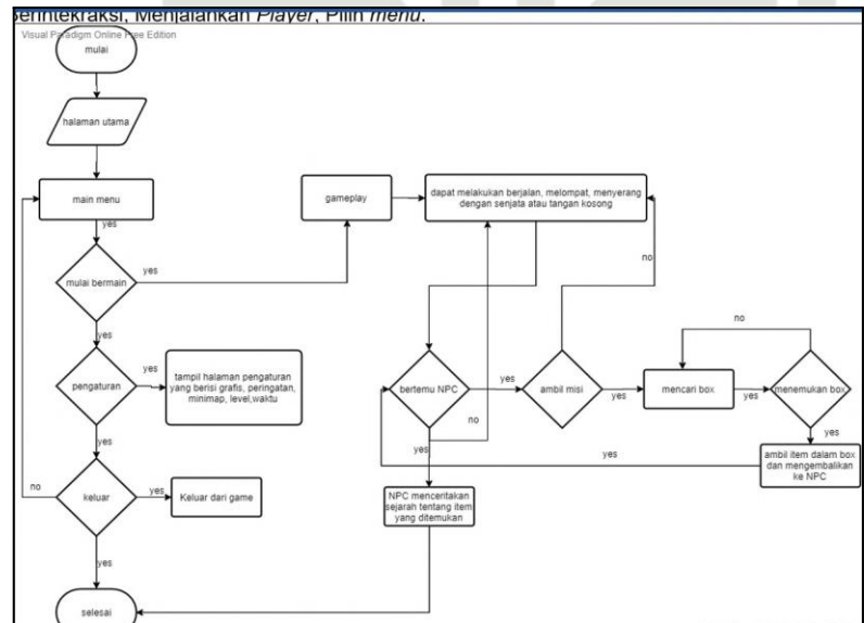
Gambar 4. Flowchart Storyboard RPG Pendekatan Balanced Design
