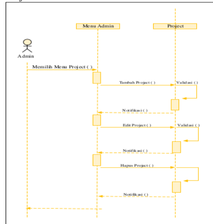
Gambar 9 Sequence diagram articlew projects
