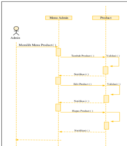
Gambar 7 Sequence diagram articlew product
