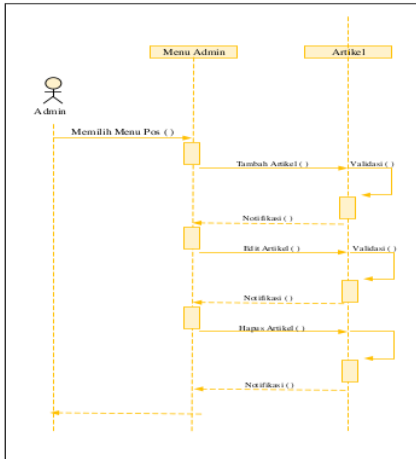
Gambar 6 Sequence diagram articlew post
