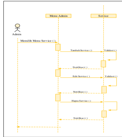
Gambar 8 Sequence diagram articlew services
