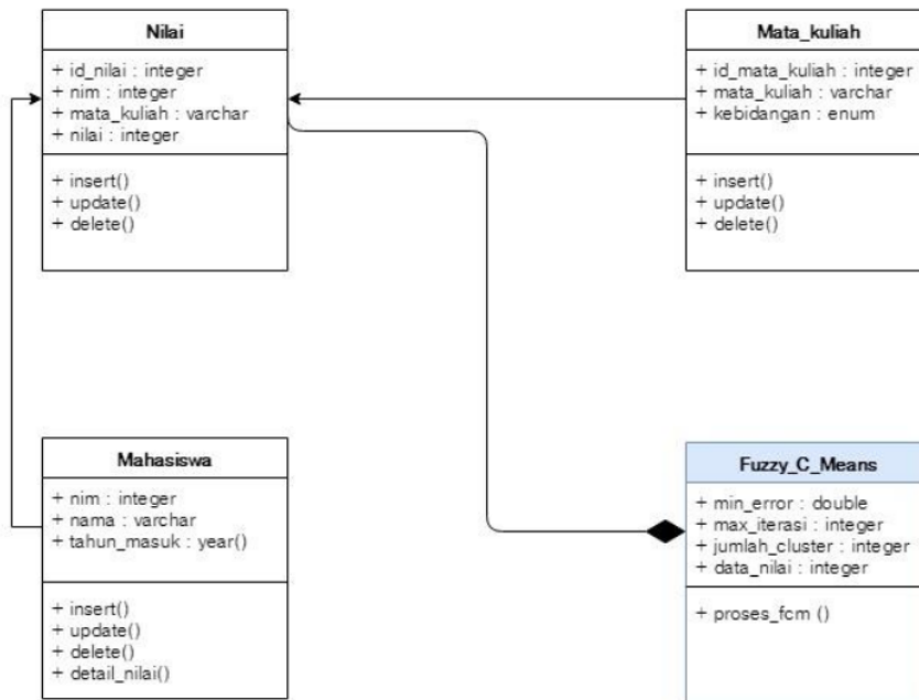
Gambar 4.3 Class Diagram
