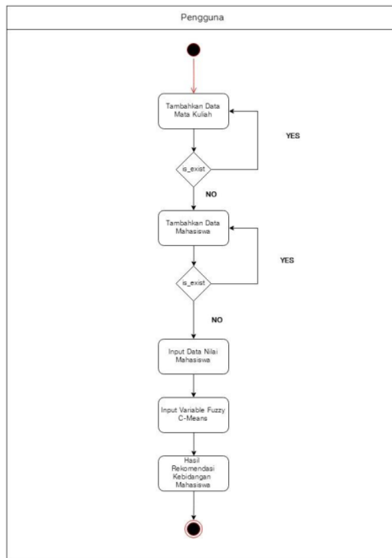
Gambar 4.4 Activity Diagram
