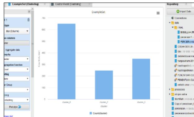
Gambar 2. Tampilan Visualizations
