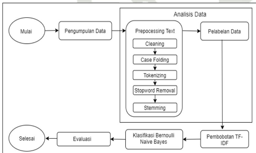
Gambar 1. Alur Penelitian
