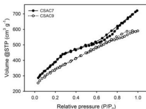
Figure 3. Nitrogen adsorption-desorption isotherms of CSAC7 and CSAC9
