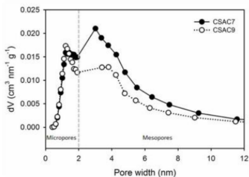
Figure 4. Pore sizes profile of CSAC7 and CSAC9
