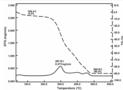
Figure 1. TG/DTG curve for pre-carbonised mission grass powder.
