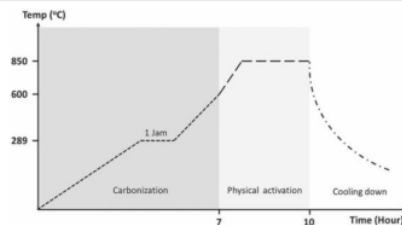
Figure 2. Profile of the one-stage integrated pyrolysis process.
