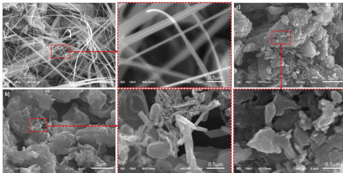
Fig. 3. SEM image for (a) TD-NaOH; (b) TD-ZnCl 2 ; and (c) TD-H 3 PO 4
