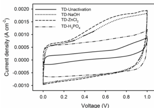
Fig. 4. CV profile of carbon coin nanofiber
