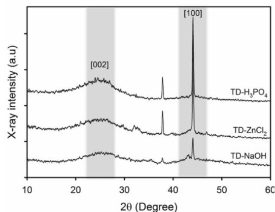
Fig. 2. XRD pattern of carbon coin nanofiber
