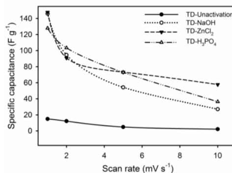
Fig. 5. Specific capacitance vs. scan rate of carbon coin nanofiber
