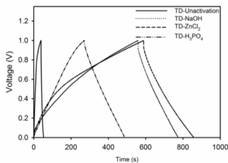
Fig. 6. GCD profile of carbon coin nanofiber
