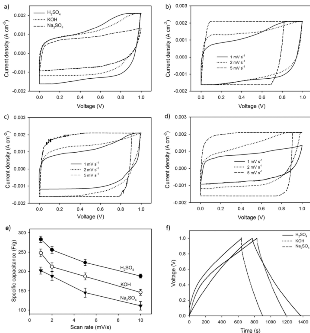
Figure 7. (a) CV curve of the MOLs750 carbon in different aqueous electrolytes, (b–d) Improved scanning was also applied to MOLs750 in different aqueous electrolytes, (e) capacitive performance of carbon MOLs in different scan rate in different aqueous electrolytes, and (f) GCD curve of the MOLs750 carbon in different aqueous electrolytes.
