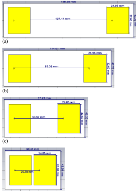
Fig. 4. Microstrip antenna design of two elements in H-plane (a) \lambda , (b) \frac{3}{4}\lambda , (c) \frac{1}{2}\lambda , (d) \frac{1}{4}\lambda .
