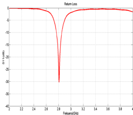
Fig. 5. Return loss (S11) and bandwidth
