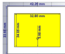
Fig.1. Single element microstrip antenna
