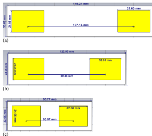
Fig.3. Microstrip antenna design of two elements in E-plane (a) \lambda , (b) \frac{3}{4}\lambda , (c) \frac{1}{2}\lambda
