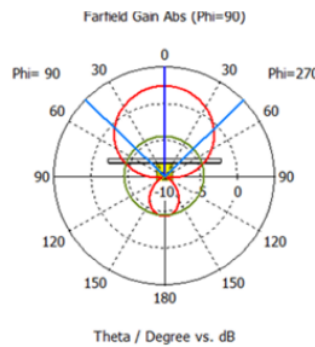
Fig. 7. SLL and beam width
