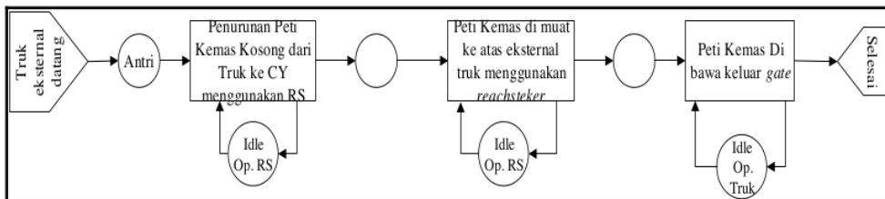
Gambar 4 ACD model 2
