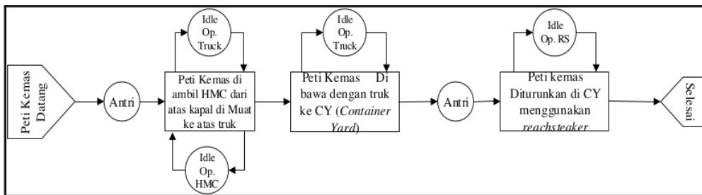
Gambar 3 ACD model 1
