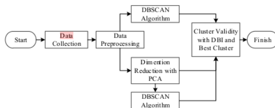
Fig. 1. Research Methodology
